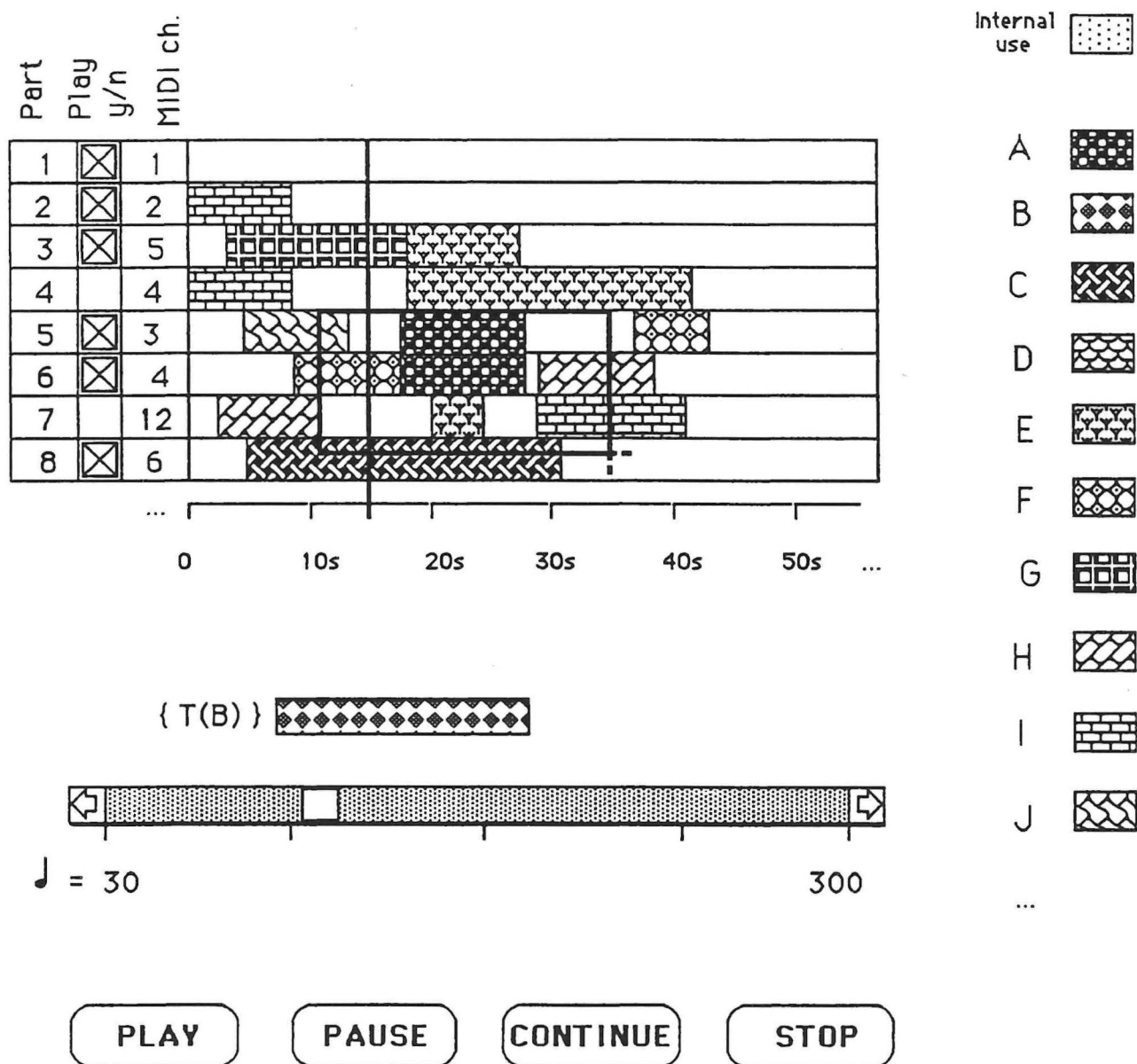
Figure 3: the main window of the FP system (Macintosh version)
